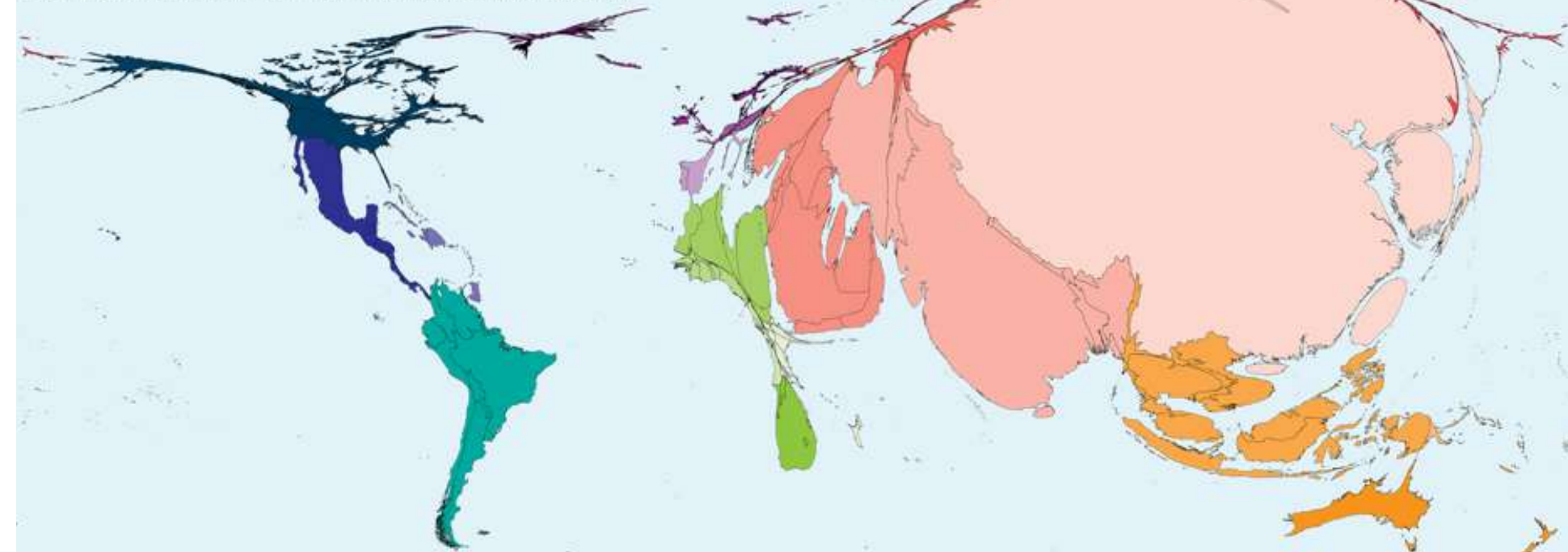
CO 2 Emissions Increase 1990-2015
